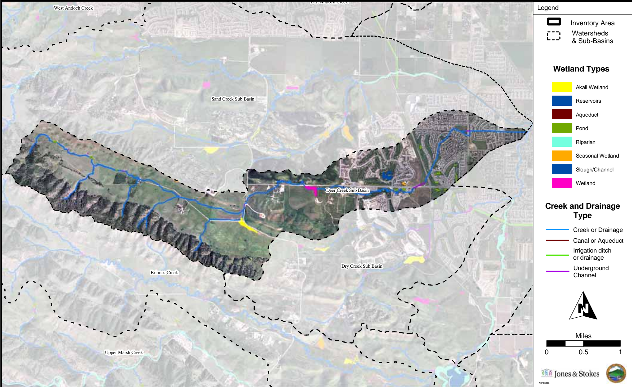
Figure 5-7a Wetland Types in Deer Creek Subbasin
