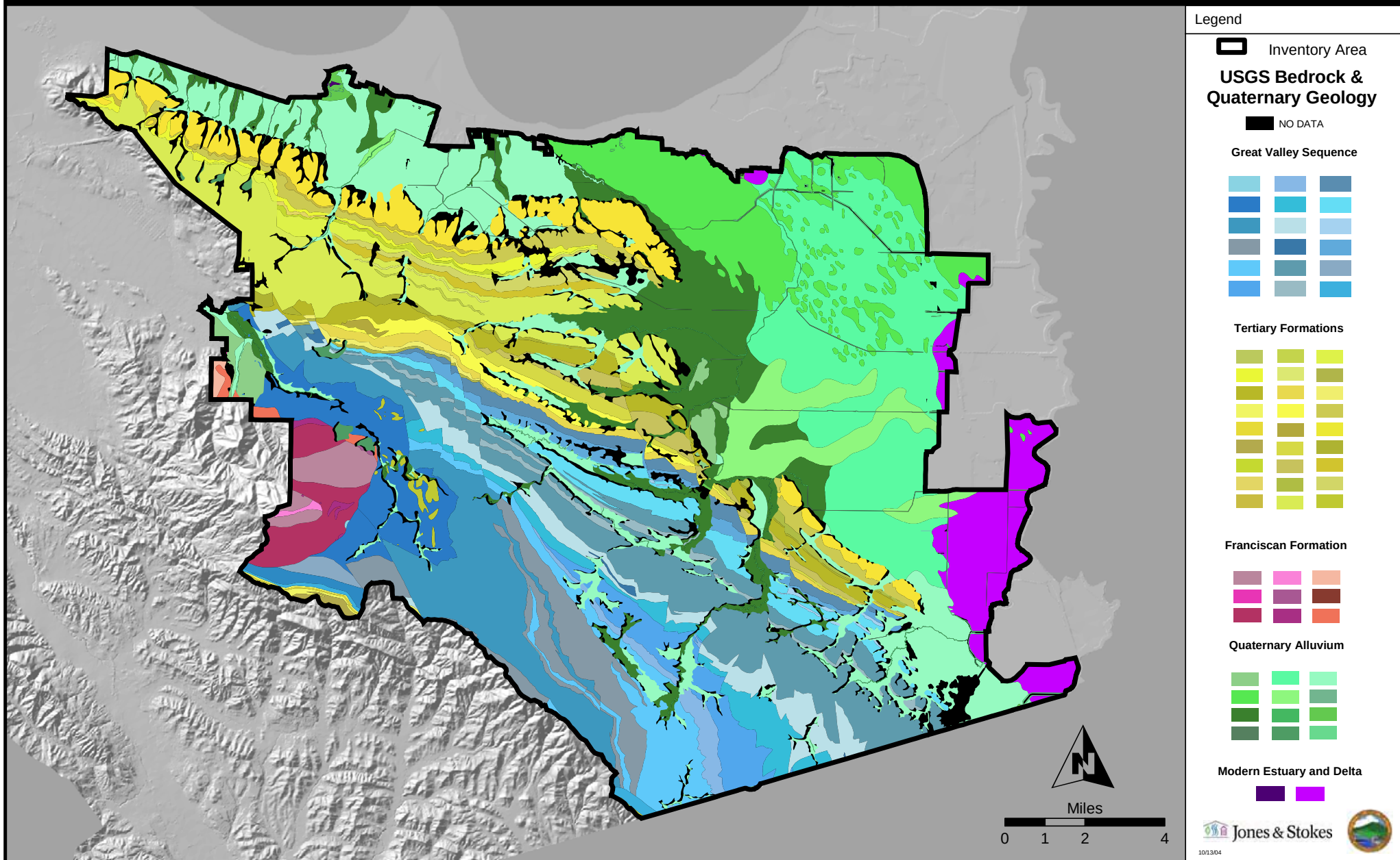
Figure 3-1 Regional Geology
