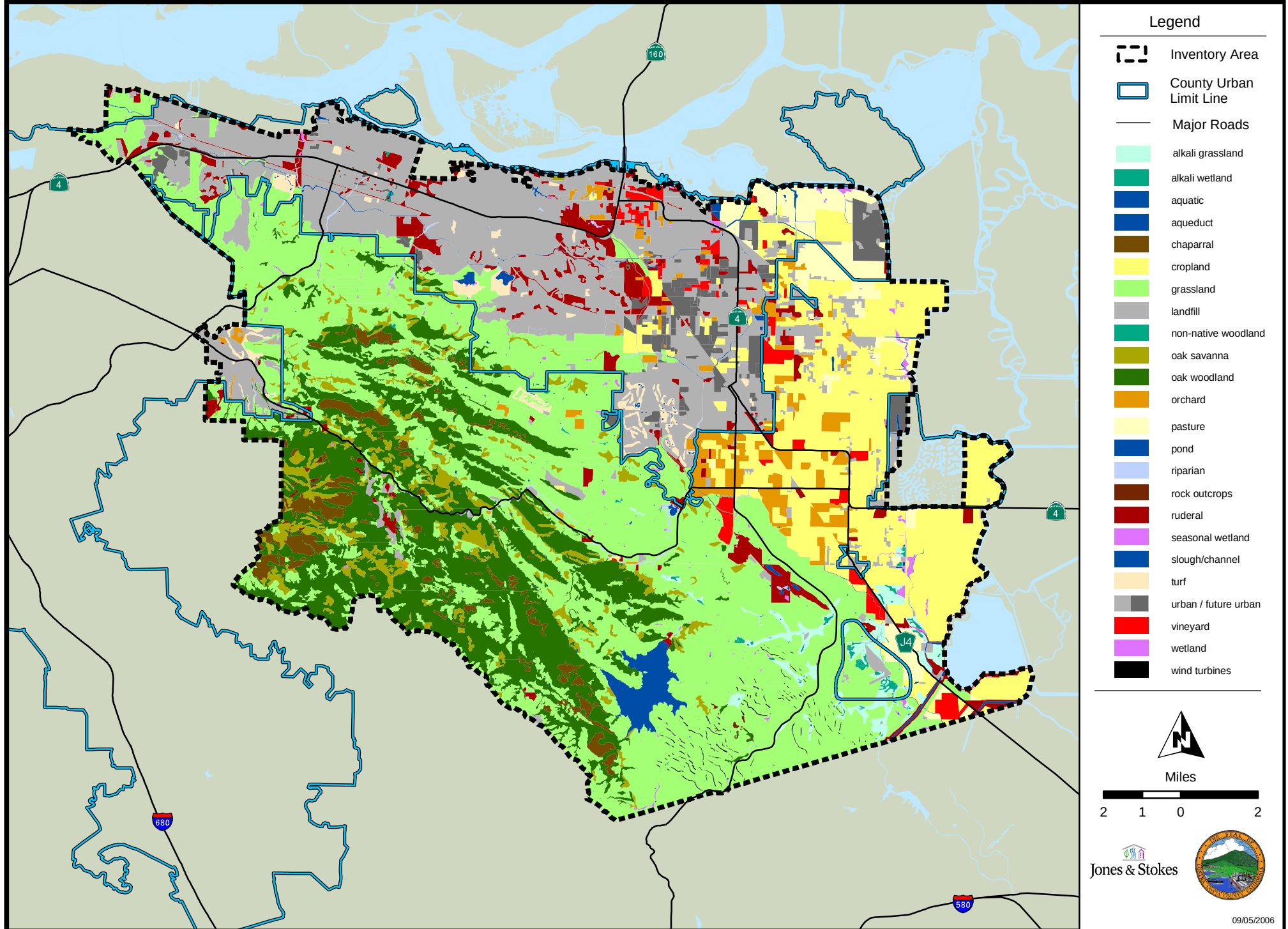
Figure 3-3 : Landcover in the Inventory Area
