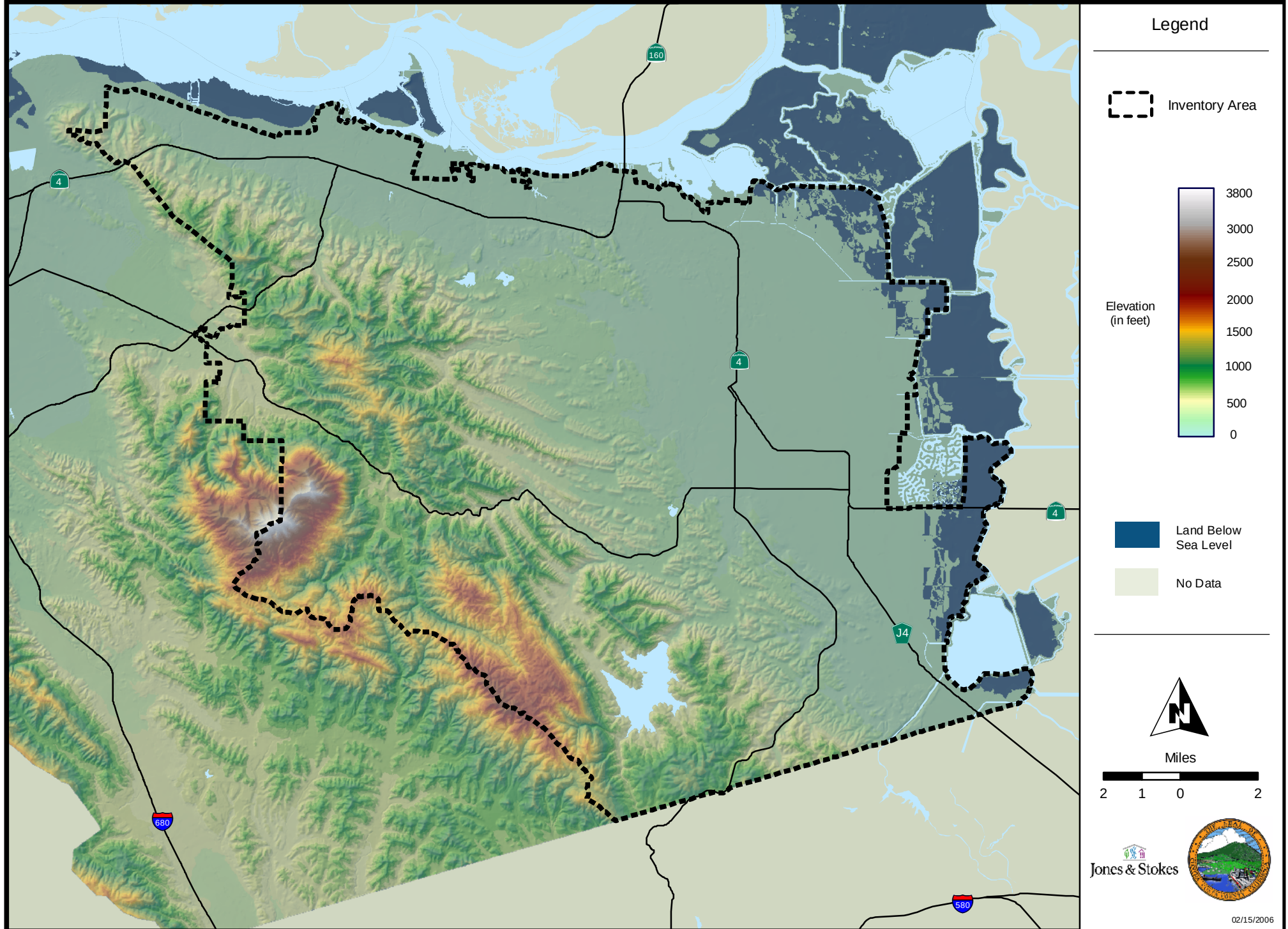
Figure 3-1 : Topography of the Inventory Area
